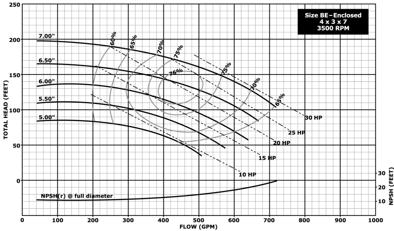
Hydraulic Performance – 7” Impeller Pumps
